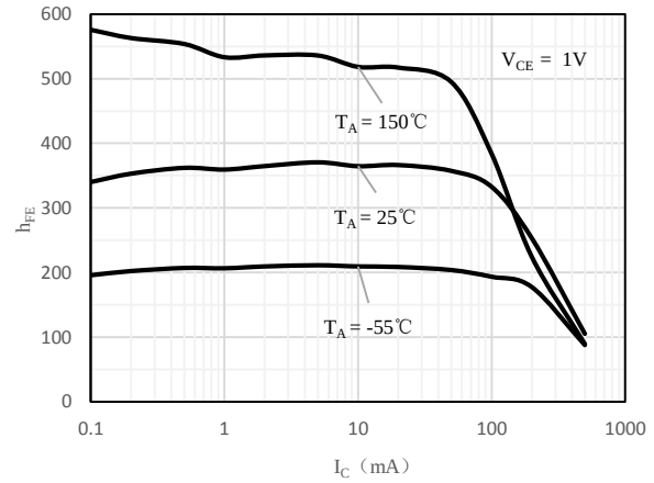
Fig 2 h_{FE} vs. I_C (BCW65B)
