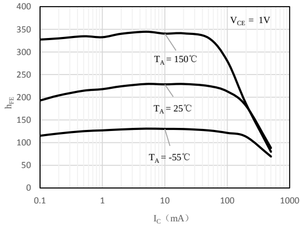
Fig 1 h_{FE} vs. I_C (BCW65A)
