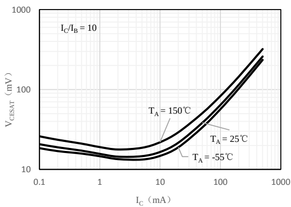
Fig 5 V_{CE(sat)} vs. I_C
