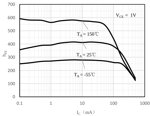
Fig 3 h_{FE} vs. I_C (BCW65C)
