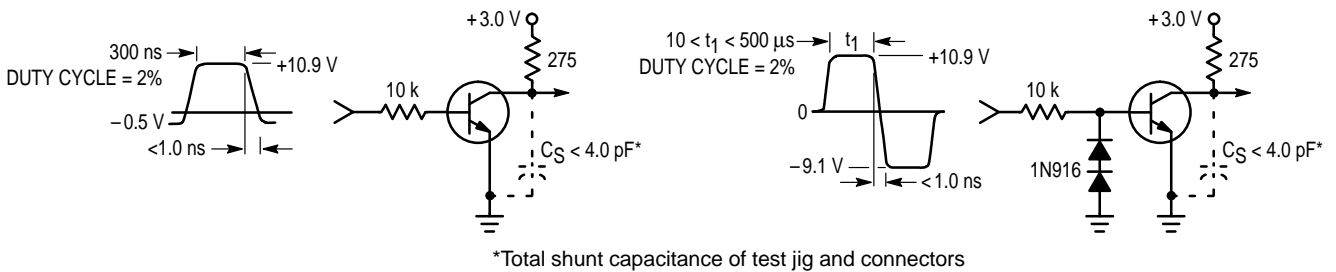
Figure 1. Turn-On Time
