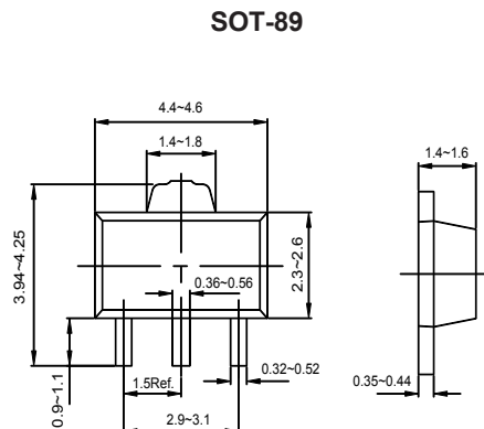
Dimension in Millimeter
