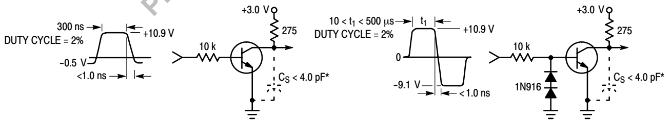
Figure 1. Turn–On Time
