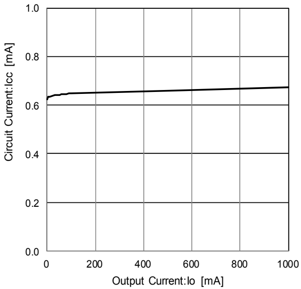
Figure 67. Circuit Current
