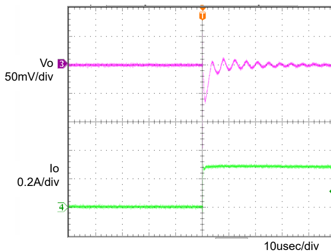
Figure 4. Transient Response (0→0.3A) Co=1\mu F , T_a=25^\circ C
