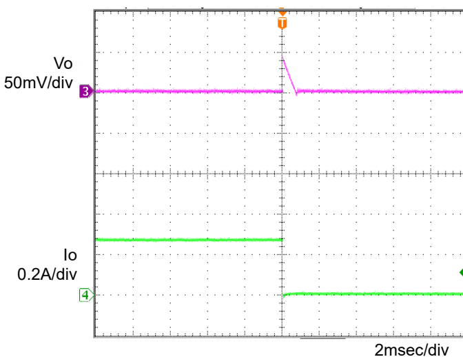
Figure 6. Transient Response (0.3→0A) Co=1\mu F , T_a=-40^\circ C
