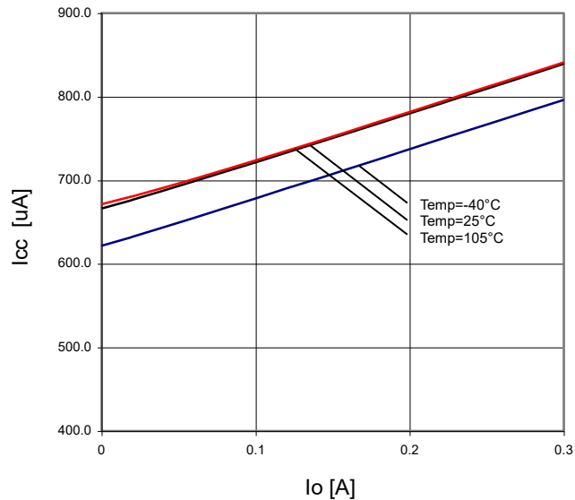
Figure 30. Io-Icc
