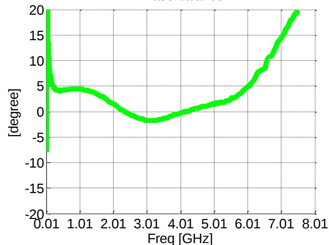
Phase balance
