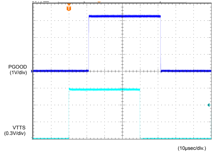
Figure 15. PGOOD Delay (TSD OFF-TSD ON)
