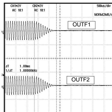
Figure 15. Advanced Switch 2
