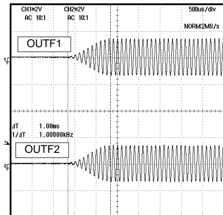
Figure 14. Advanced Switch 1
