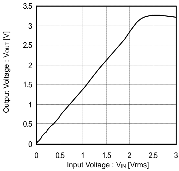
Figure 21. Output Voltage vs Level Meter V_{IN}
