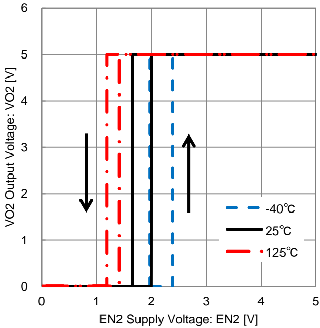
Figure 20. VO2 Output Voltage vs EN2 Supply Voltage (EN2 Threshold Voltage)
