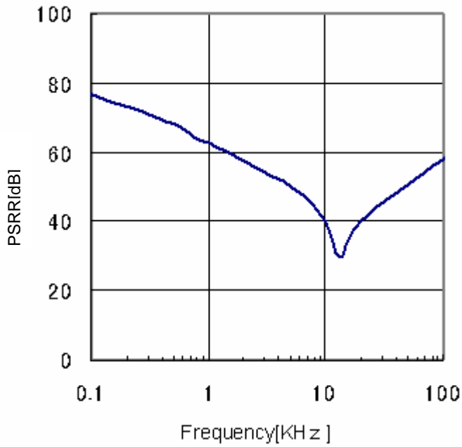
Fig.20 PSRR ( I_o=0mA )
