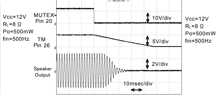
Fig. 14 Wave form when Activating Soft-mute
