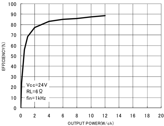
Fig.17 Output power—Efficiency ( R_L=6\Omega )
