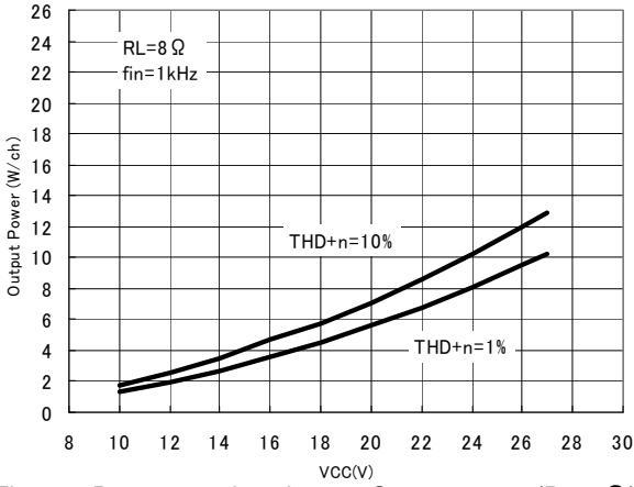
Fig.13 Power supply voltage—Output power ( R_L=8\Omega )
