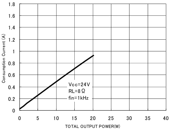
Fig.15 Total output power—Current consumption ( R_L=8\Omega )
