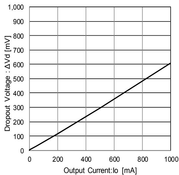
Figure 40. Dropout Voltage ( V_{cc}=V_o \times 0.95V )
