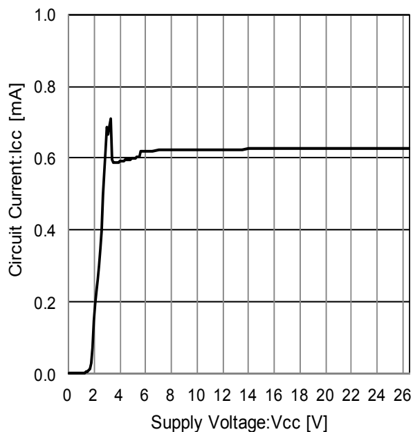
Figure 24. Circuit Current
