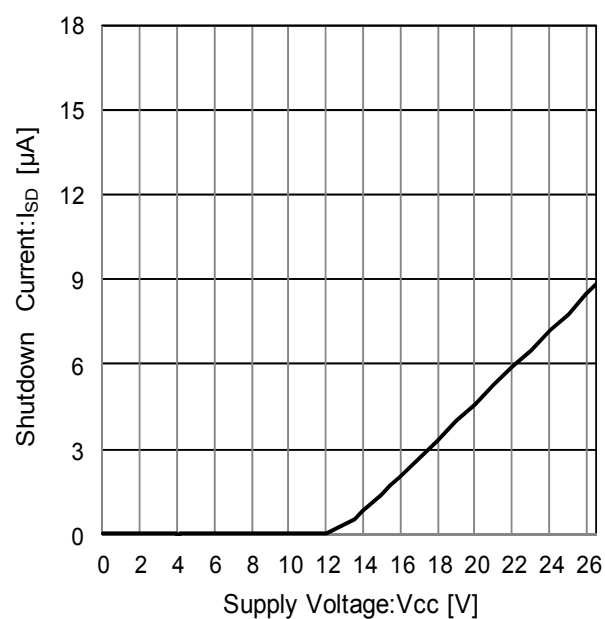
Figure 60. Shutdown Current
