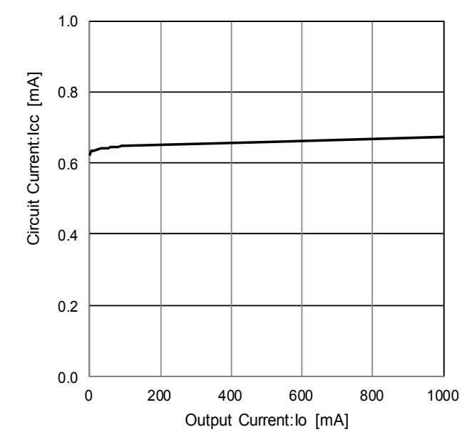
Figure 67. Circuit Current
