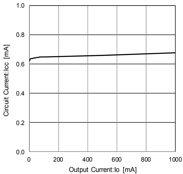
Figure 43. Circuit Current
