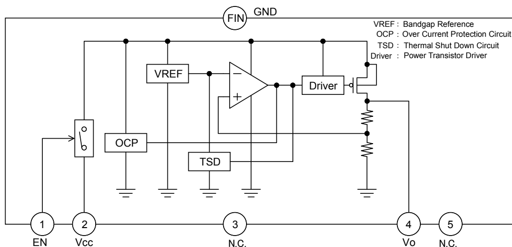
Figure 11. Block diagram BDxxFC0WFP (Output Voltage Fixed Type, with Shutdown SW)
