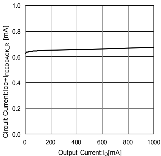
Figure 20. Circuit Current ( I_O = 0\text{mA} \rightarrow 1000\text{ mA} ) ( I_{FEEDBACK\_R} \approx 75\mu\text{A} )
