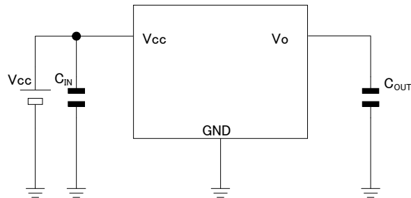
Figure 3. Typical Application Circuit Output Voltage Fixed Type (Without Shutdown SW)
