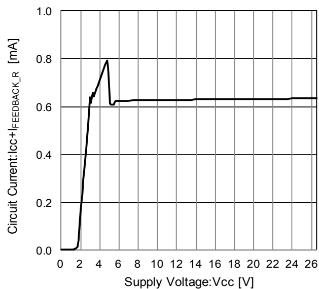
Figure 12. Circuit Current ( I_{FEEDBACK\_R} \approx 75\mu\text{A} )
