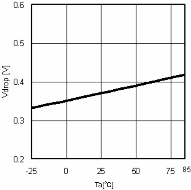
Fig.18 Minimum dropout Voltage1 (V CC =5V、I O =-0.5A)
