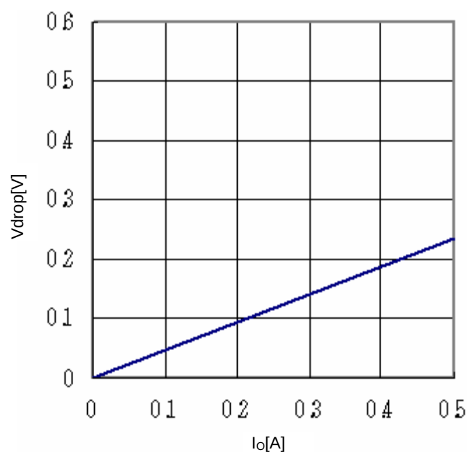
Fig.26 Minimum dropout Voltage 6 ( V_{CC}=12V , T_a=25^\circ C )
