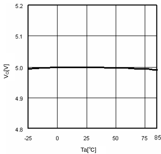
Fig.9 T_a - V_O ( I_o=0mA )
