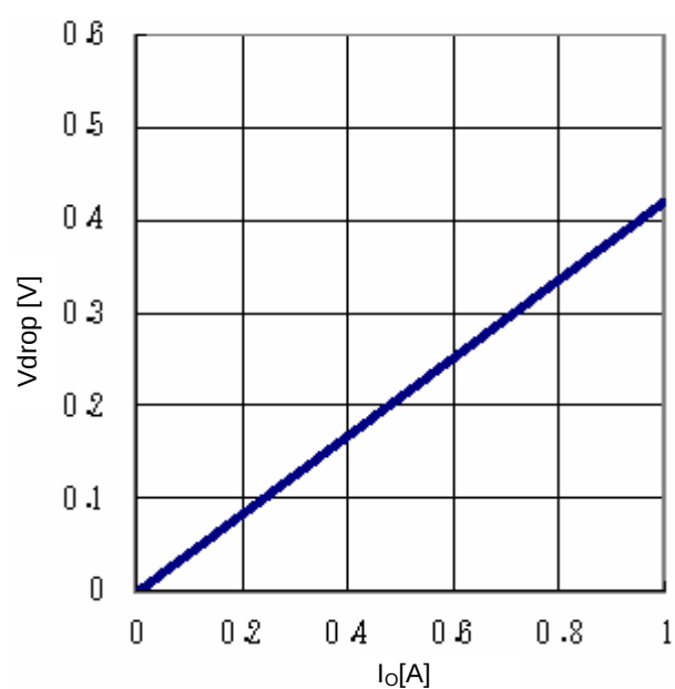
Fig.22 Minimum dropout Voltage 3 ( V_{CC}=6V , T_a=25^{\circ}C )
