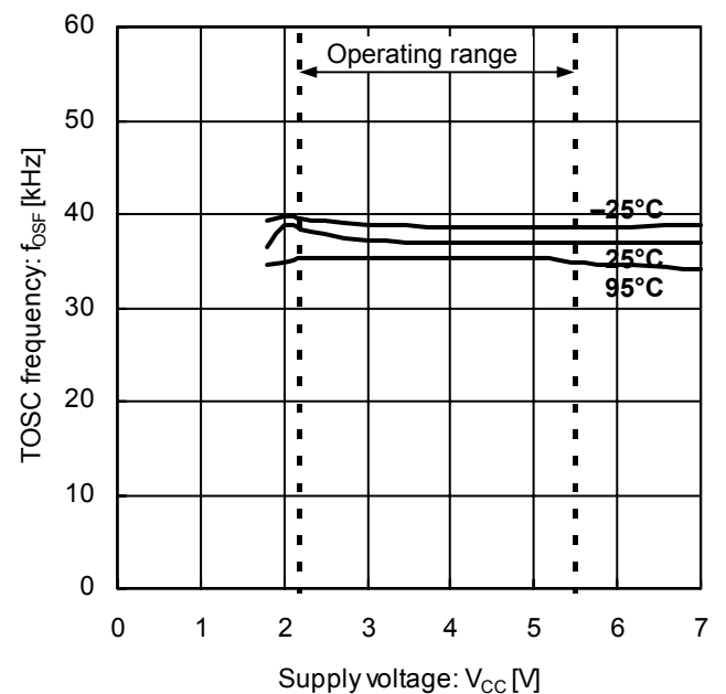
Figure 6. TOSC frequency
