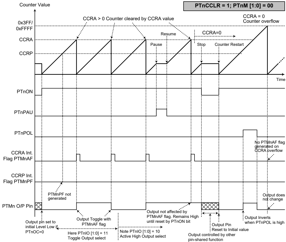
Compare Match Output Mode – PTnCCR=1 (n=0~3)
