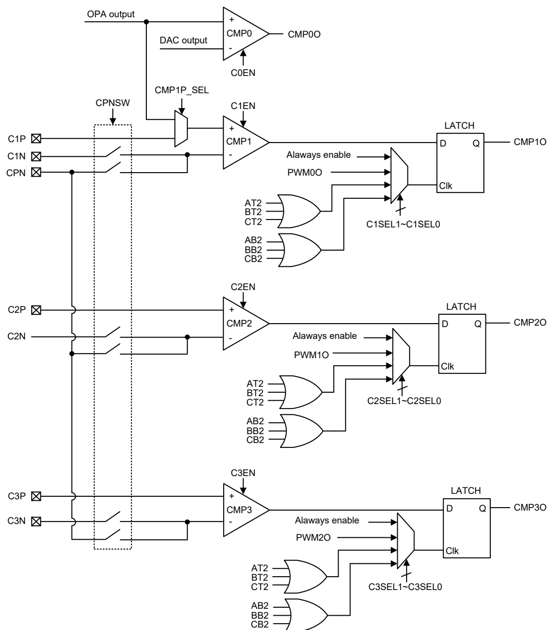
Comparator Block Diagram
