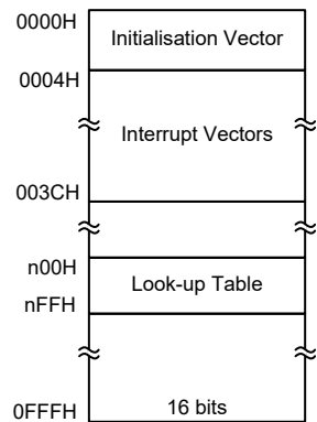
Program Memory Structure
