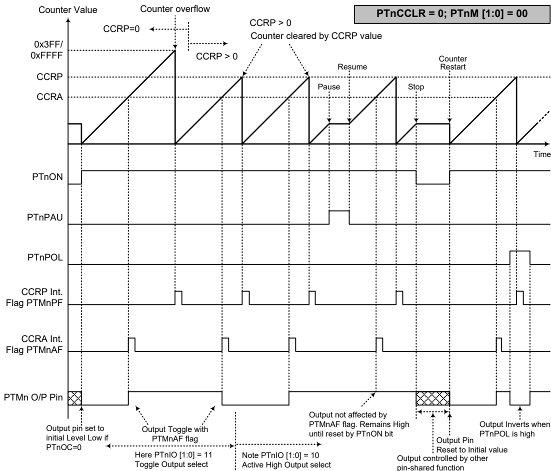
Compare Match Output Mode – PTnCLLR=0 (n=0~3)
