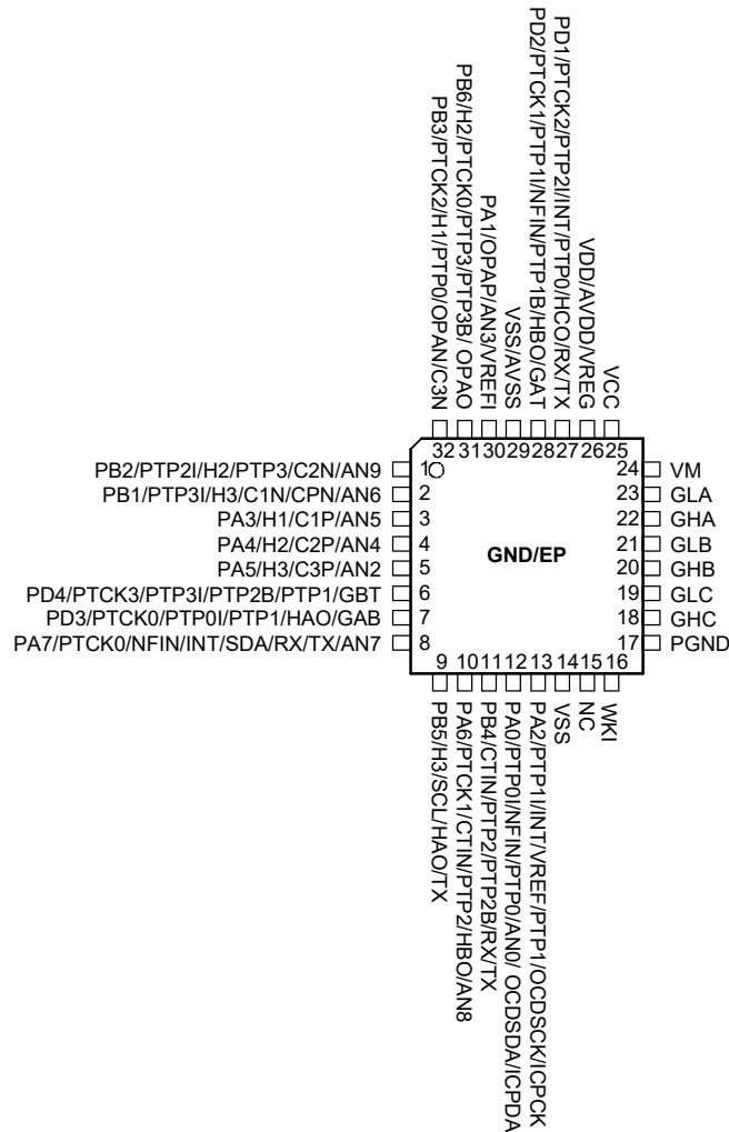
BD66FM6452A/BD66VM6452A 32 QFN-A
