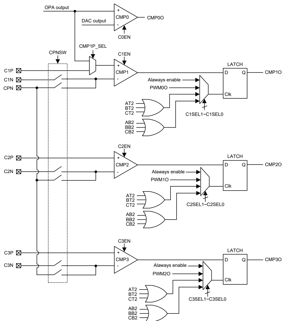
Comparator Block Diagram
