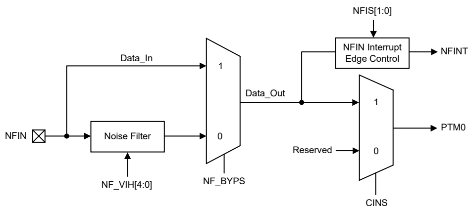
Digital Noise Filter Block Diagram
