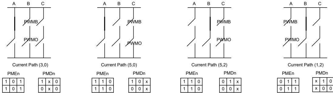
Mask Complement Mode Examples
