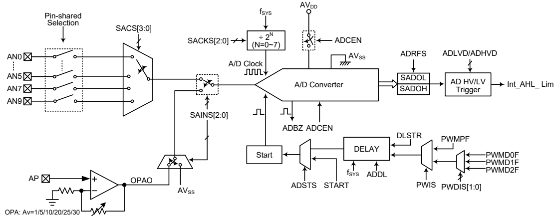
A/D Converter Structure
