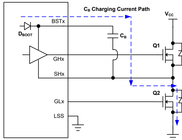
Bootstrap Capacitor ( C_B ) Charging Current Path
