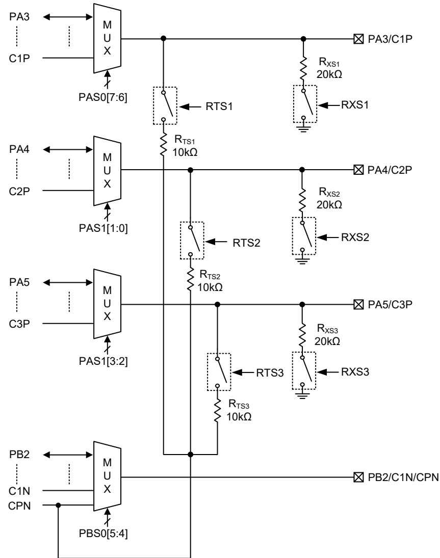
BEMF Detector Block Diagram
