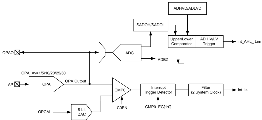
Over Current Detection Block Diagram
