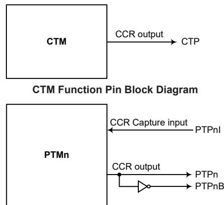
PTMn Function Pin Block Diagram (n=0~1)
