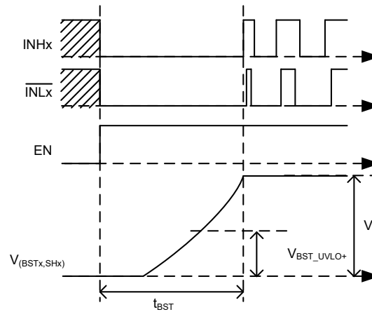
Bootstrap Capacitor Charging Time ( t_{BST} )
