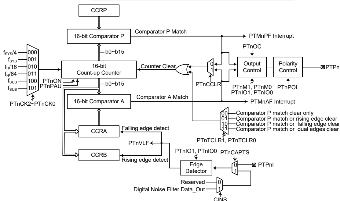
16-Bit Periodic Type TM Block Diagram (n=0)
