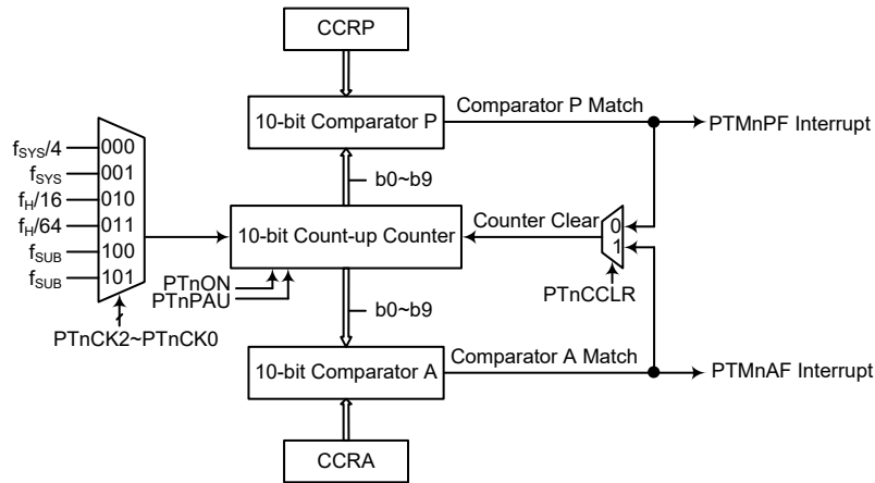
10-Bit Periodic Type TM Block Diagram (n=2~3)
