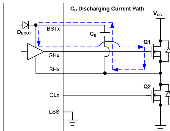
Bootstrap Capacitor ( C_B ) Discharging Current Path
