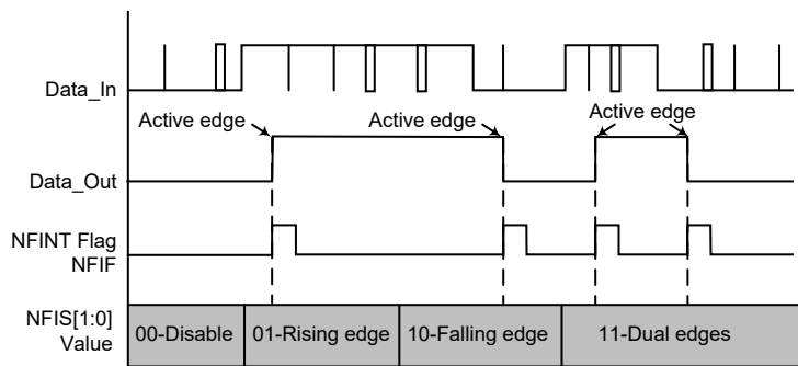
Digital Noise Filter Interrupt Trigger
