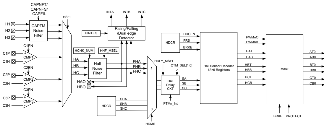
Hall Sensor Decoder Block Diagram
