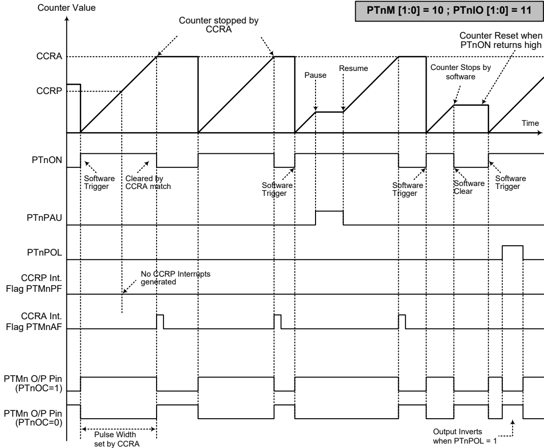
Single Pulse Output Mode (n=0~1)
