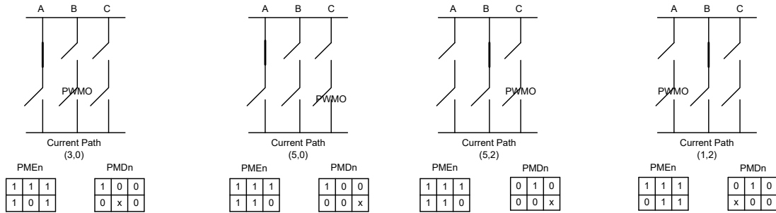
Mask Independent Mode Examples
