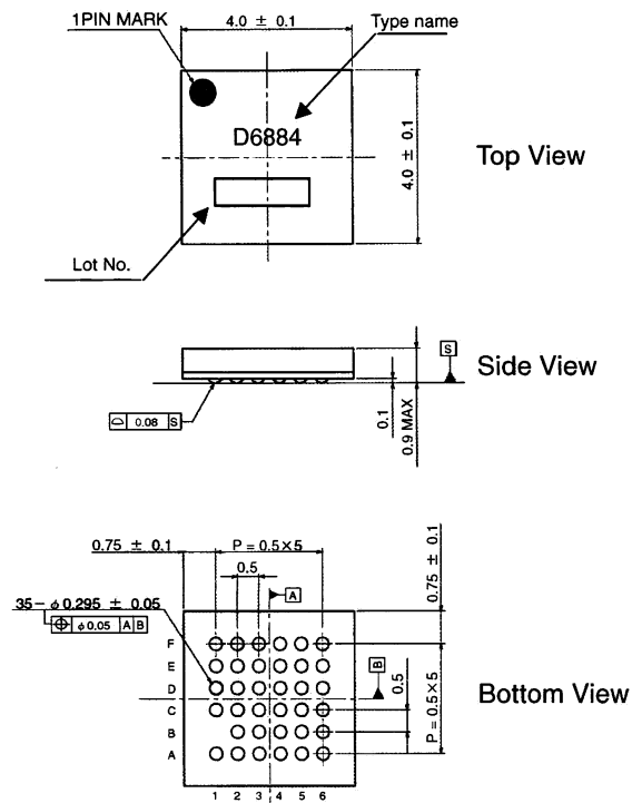
Fig.1 VBGA035W040 Package (Unit: mm)
