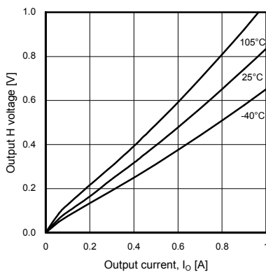
Figure 8. Output H Voltage (Temperature Characteristics)
