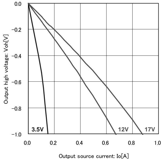
Fig.6 Output high voltage (Ta=25°C)
