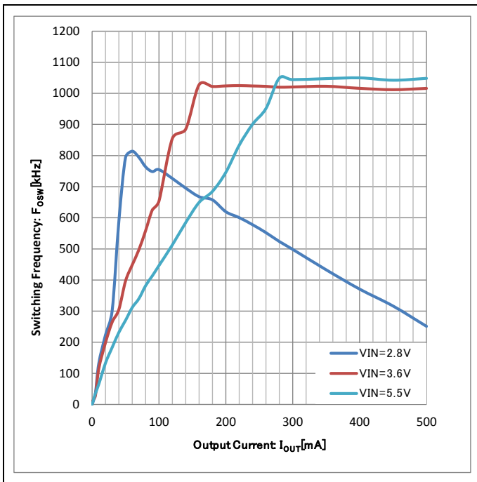
Figure 17. Switching Frequency vs Output Current (VOUT=2.5V)
