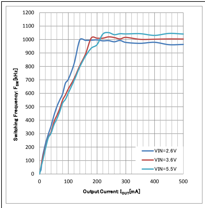
Figure 15. Switching Frequency vs Output Current (VOUT=1.2V)
