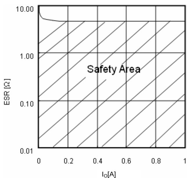
Fig.18 ESR condencer
