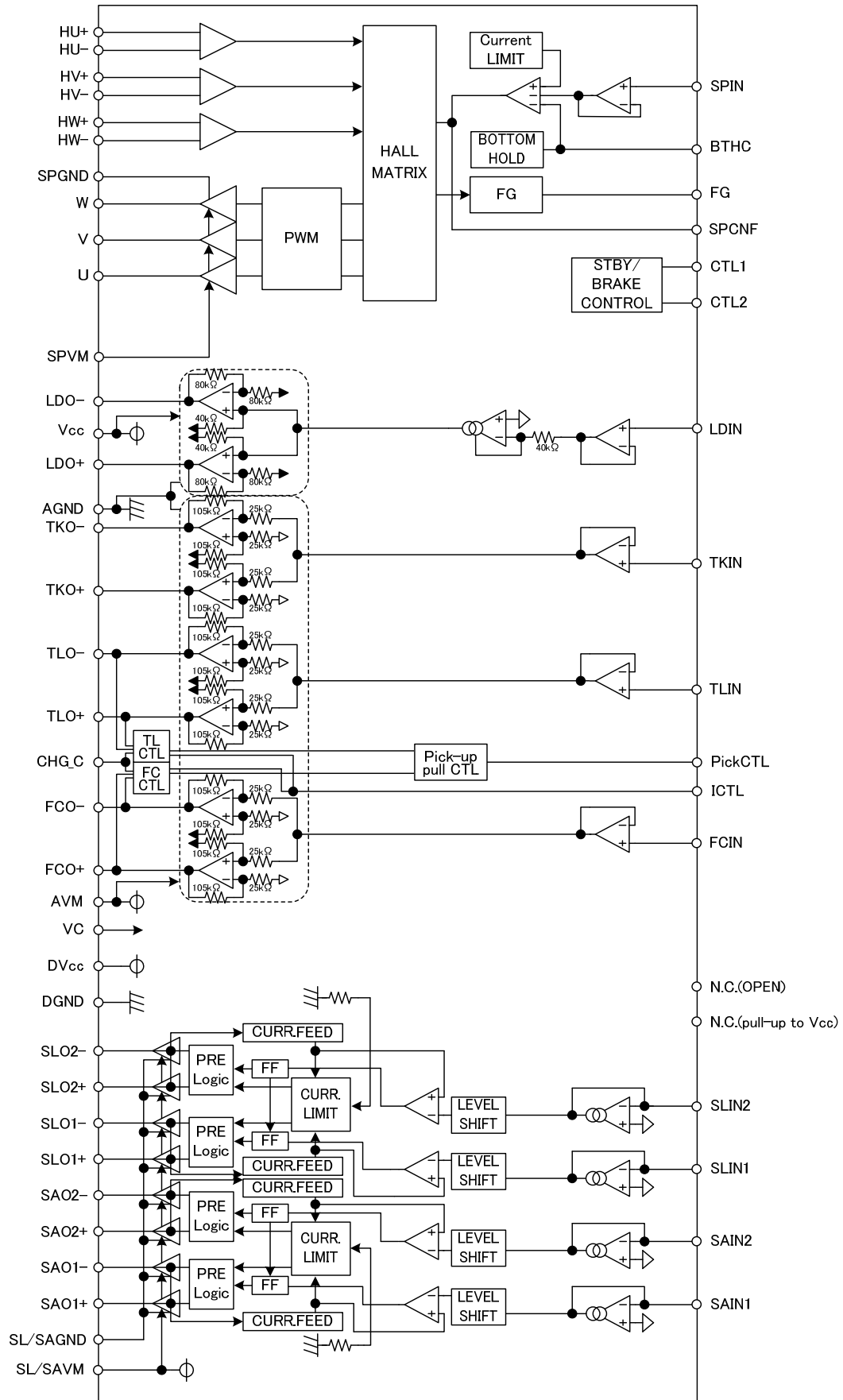
OBLOCK diagram
