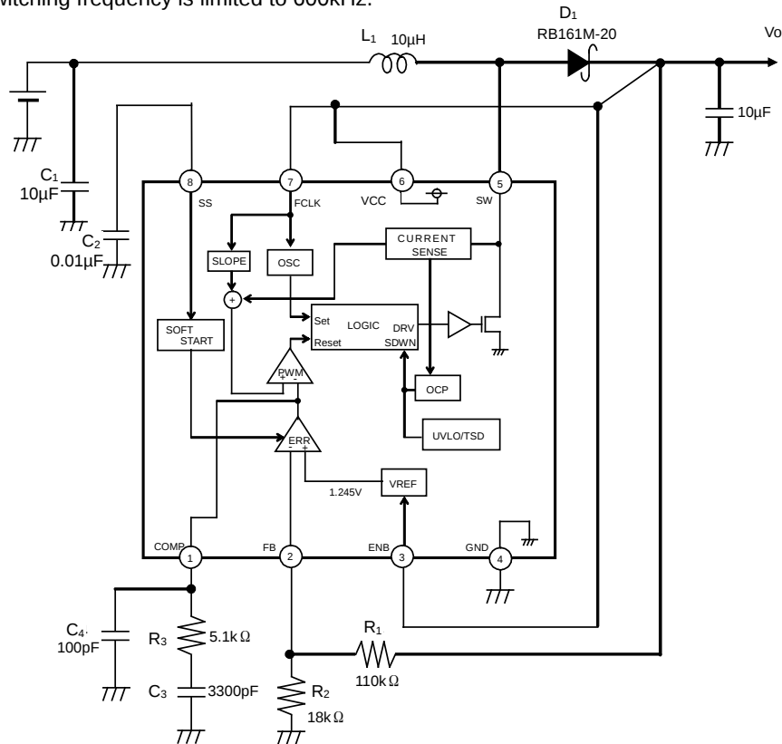
Figure 35. Circuit Diagram Example (Supply Voltage over 4.0 V)
