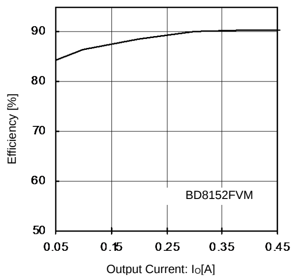
Figure 15. Efficiency vs Output Current ( V_{CC}=5V )
