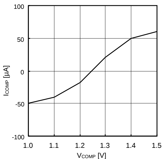
Figure 12. I_{COMP} vs V_{COMP}
