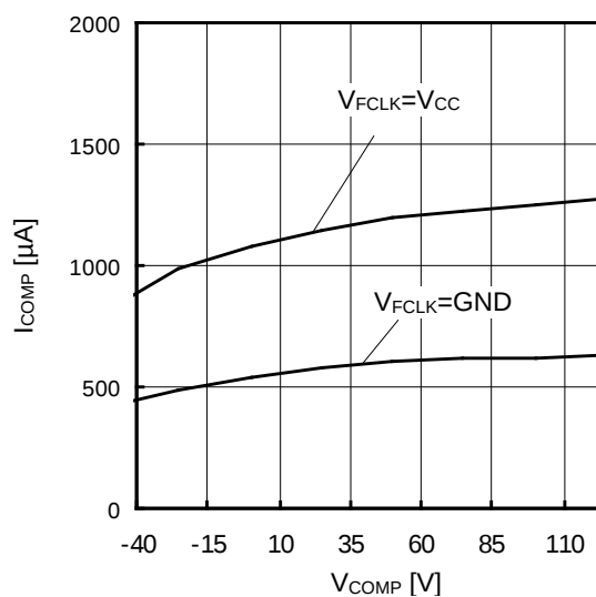
Figure 9. I_{COMP} VS V_{COMP}
