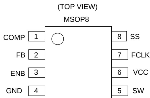
Figure 2. Pin Configuration
