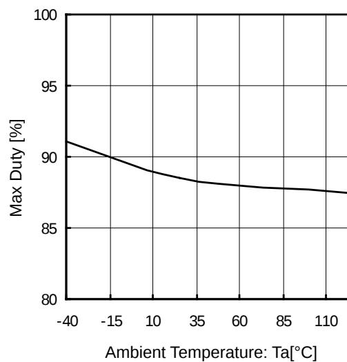
Figure 13. Max Duty vs Temperature
