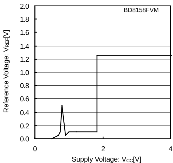
Figure 8. Reference Voltage vs Supply Voltage
