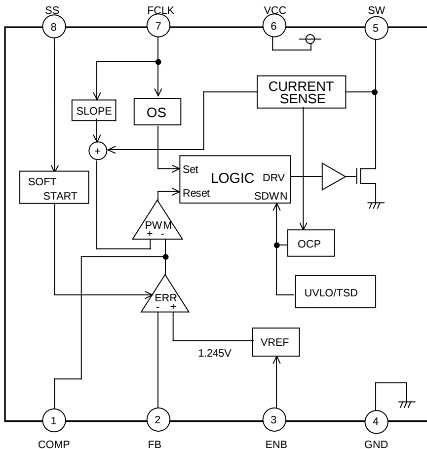
Figure 3. Block Diagram
