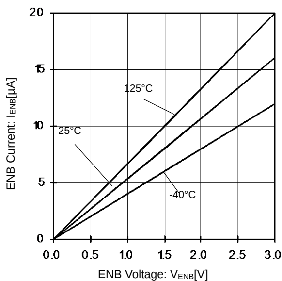
Figure 11. ENB Pin Current vs ENB Voltage
