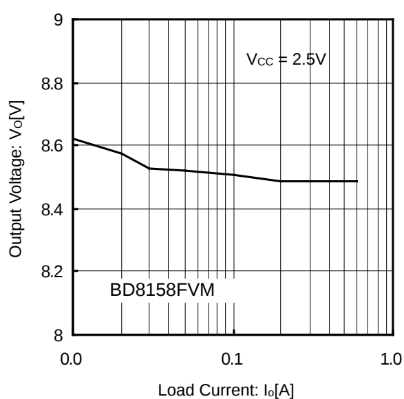
Figure 19. Output Voltage vs Load Current (Load Regulation 1)
