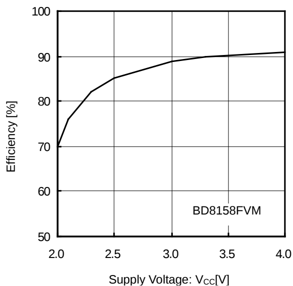
Figure 16. Efficiency vs Supply Voltage
