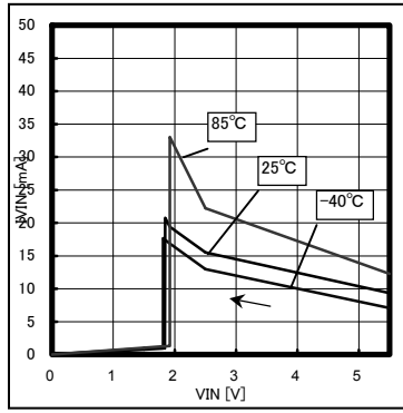
Fig.2 Curcuit Current (Switching)
