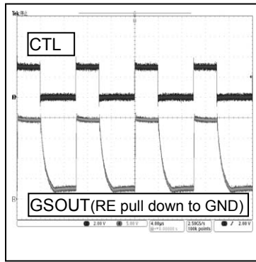
Fig.17 Gate Sharding Wave form2
