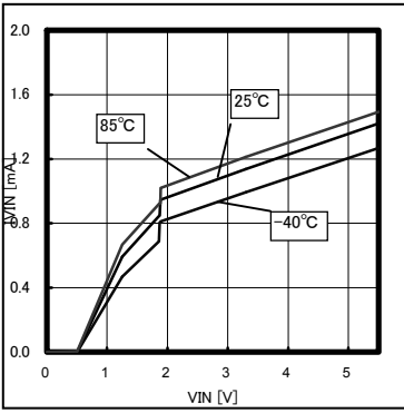
Fig.1 Curcuit Current (No switching)
