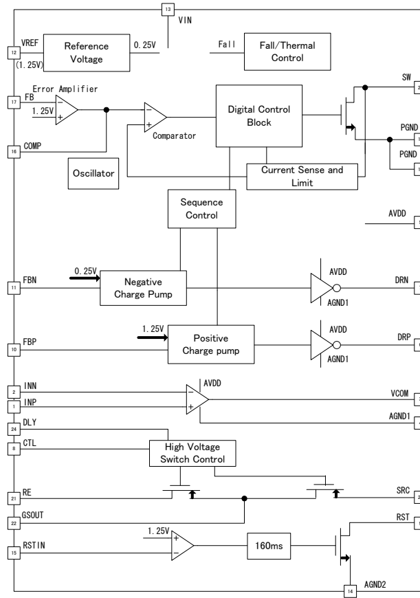
Fig.23 Block Diagram
