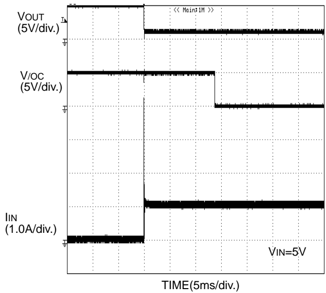
Figure 37. Over-Current Response 1 \Omega Load Connected at Enable
