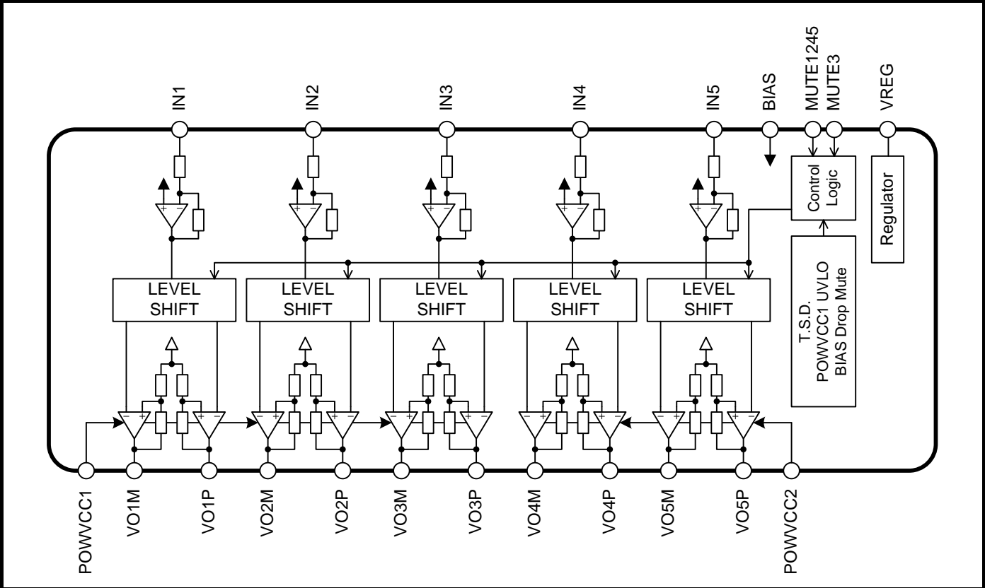
Figure 3. Block Diagram
