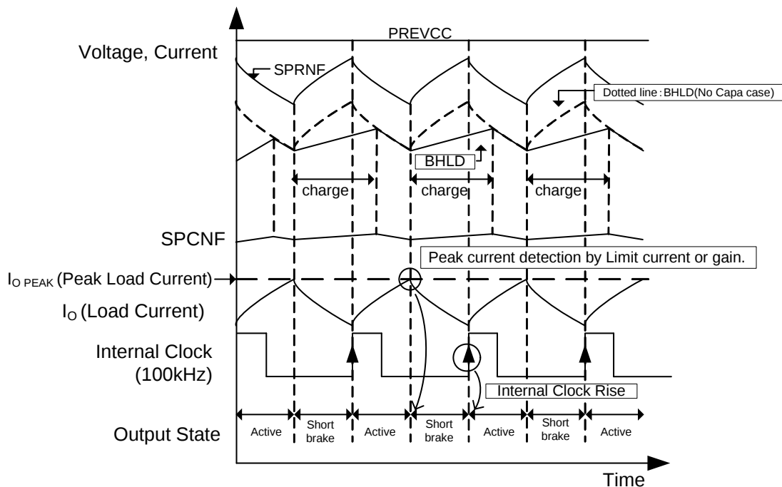
Figure 20. Spindle Driver Operation Timing Chart
