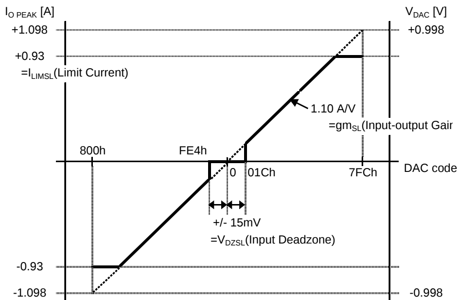
Figure 12. I_{O\text{ PEAK}} Characteristics (When set as R_{\text{SLRNF}}=0.56 \Omega ).
