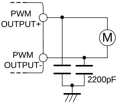
Figure 28. Snubber Circuit
