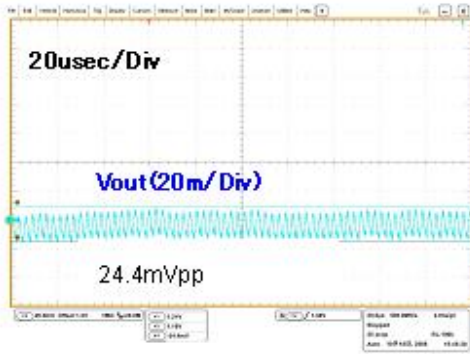
Figure 45. Output Ripple 1 (V CC =12V, I o =40mA)
