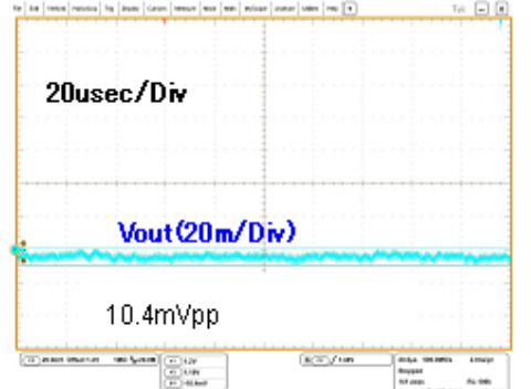
Figure 48. Output Ripple 4 (V CC =12V, I o =170mA)
