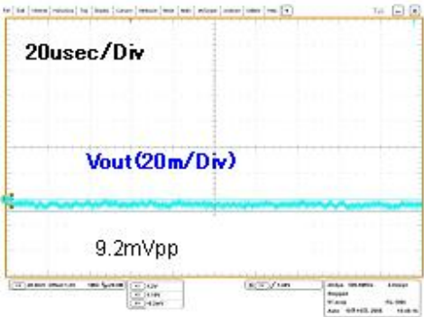
Figure 47. Output Ripple 3 (V CC =12V, I o =140mA)
