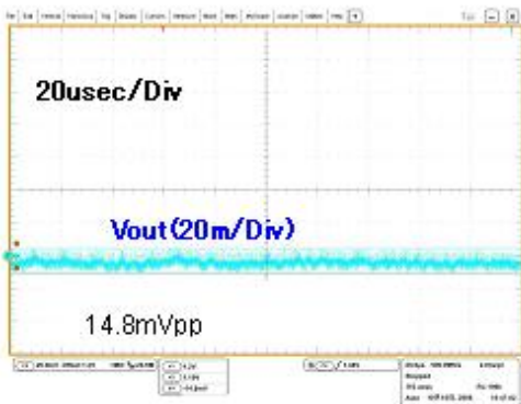
Figure 49. Output Ripple 5 (V CC =12V, I o =900mA)
