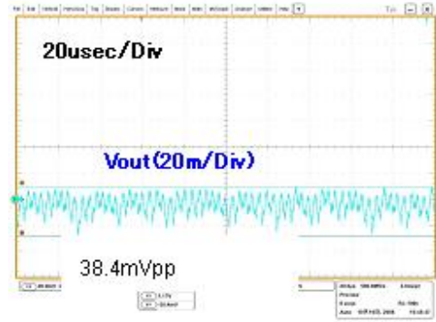
Figure 46. Output Ripple 2 (V CC =12V, I o =100mA)
