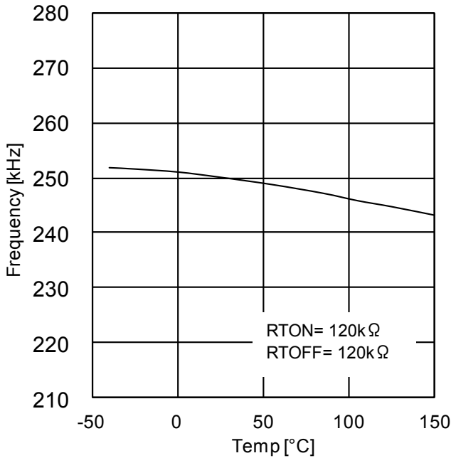
Fig.8 Frequency - Temp
