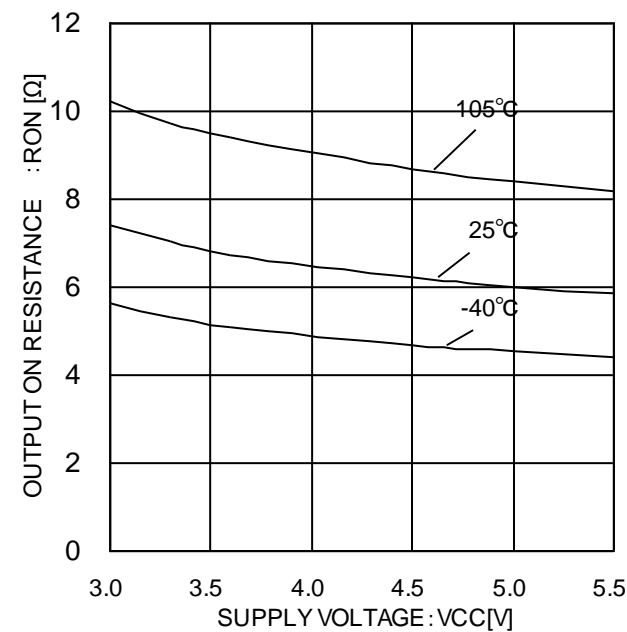
Figure 6. Output ON resistance (VCC characteristic @ ID=20mA)
