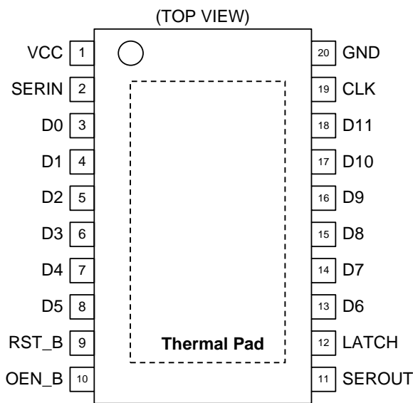
Figure 2. Pin Configuration
