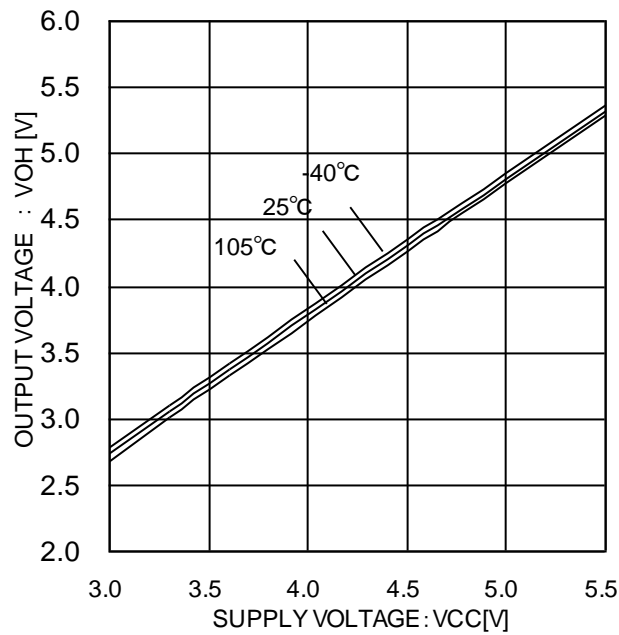
Figure 9. SEROUT high side voltage (VCC characteristic @ ISO=-4mA)
