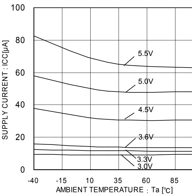
Figure 5. Circuit current (Temperature characteristic)
