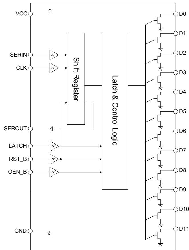
Figure 3. Block Diagram
