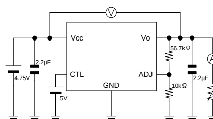
Measurement setup for Figure 13.
