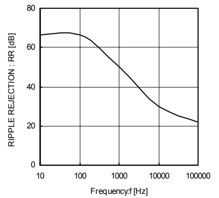
Fig. 7 Ripple Rejection
