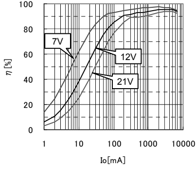
Fig.14 Efficiency ( V_o=5V , QLLM)
