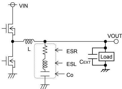
Output Capacitor
