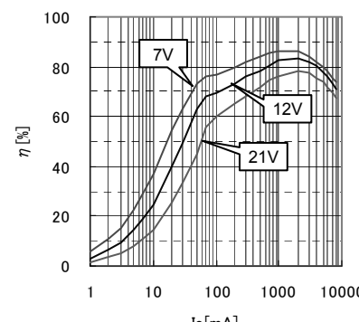
Fig.20 Efficiency ( V_o=1V , QLLM)
