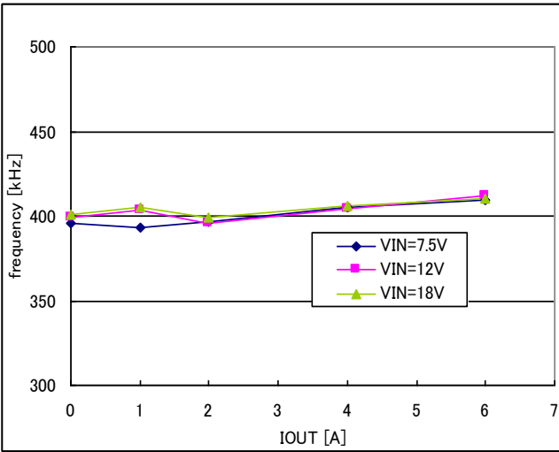
Figure 48. I o -frequency (V o = 3.3V, PWM, RFS= 68kΩ)
