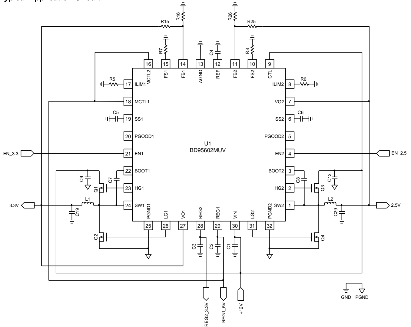
Figure 1. Application Circuit
