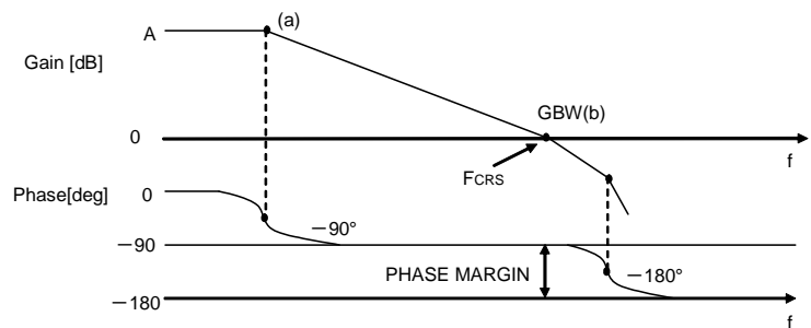
Figure 52. Bode Plot
