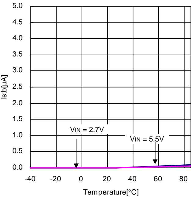
Figure 5. Stand-by Current vs Temperature
