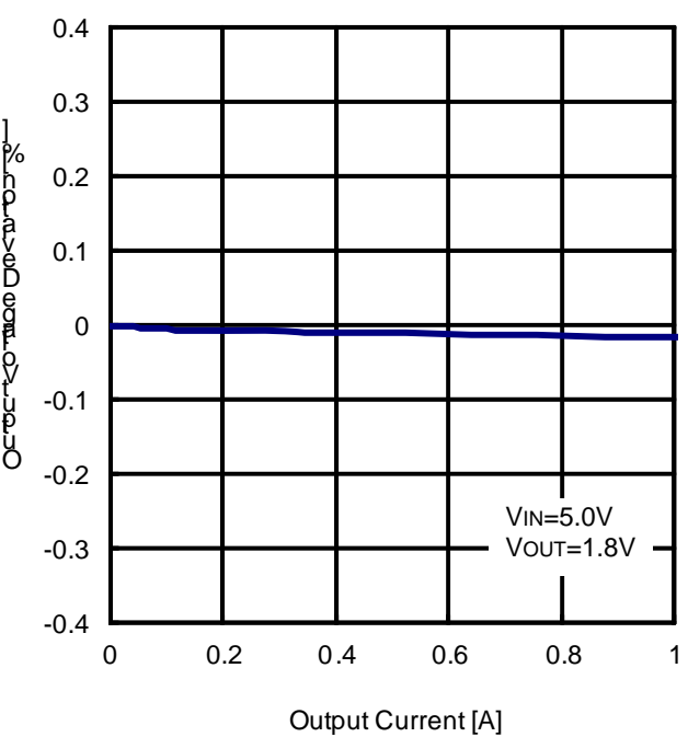
Figure 38. Load Regulation vs Load Current
