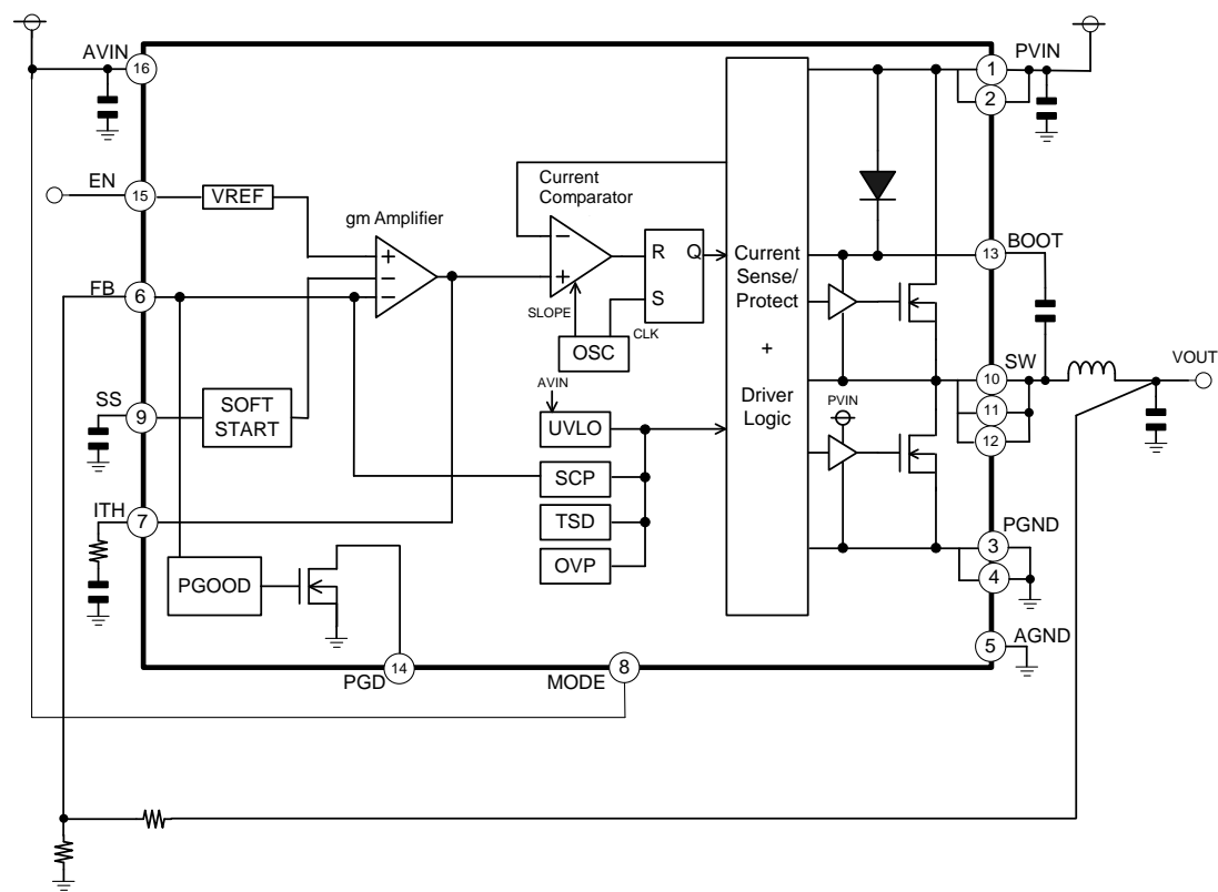
Figure 3. Block Diagram
