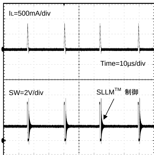
Figure 36. Switching Waveform with SLLM™ ( V_{IN} = 3.3V , V_{OUT} = 1.8V , I_{OUT} = 30mA , L = 1.5\mu H )
