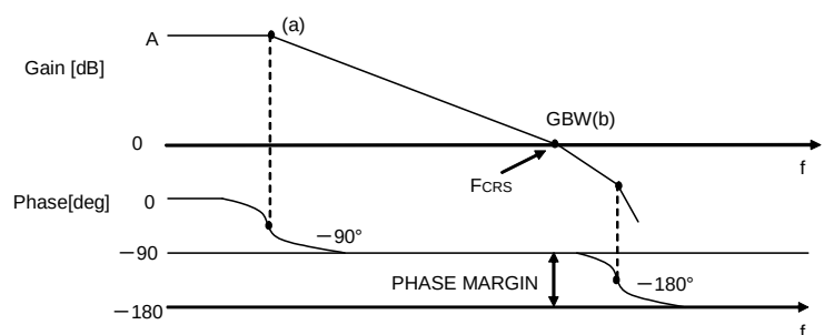
Figure 53. Bode Plot
