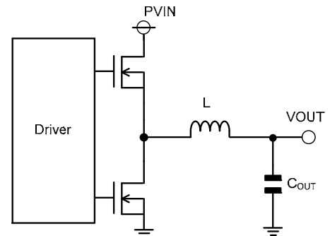
Figure 50. Output LC filter circuit
