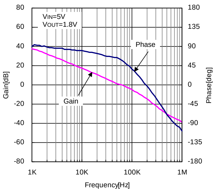
Figure 25. Closed Loop Response ( V_{IN}=5V , V_{OUT}=1.8V , I_{OUT}=1A , L=1.5\mu H , C_{OUT}=\text{Ceramic } 44\mu F )
