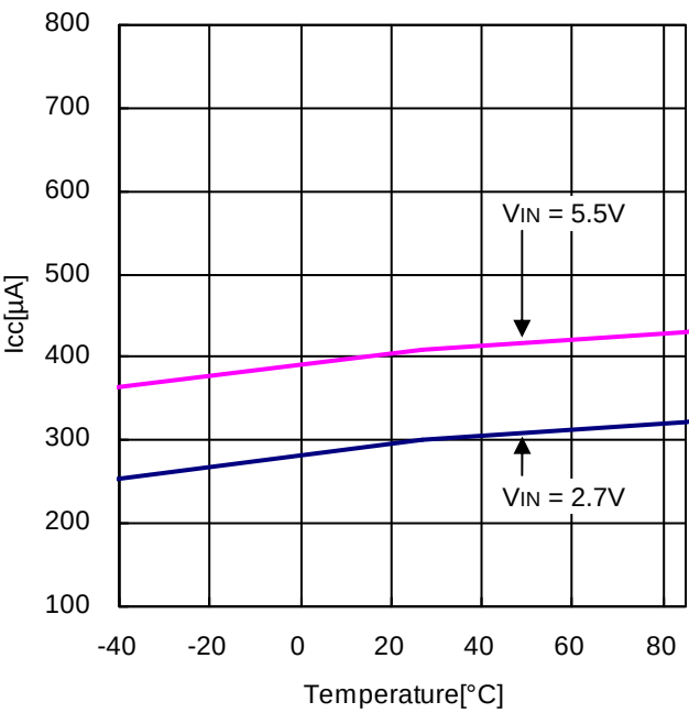
Figure 4. Operating Current vs Temperature
