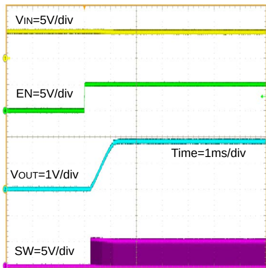
Figure 28. Power Up ( EN= 0V \rightarrow 5V )
