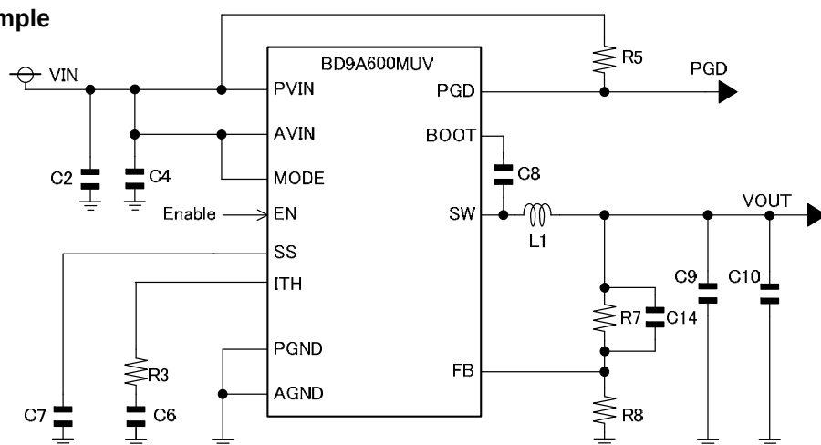
Figure 48. Application Circuit
