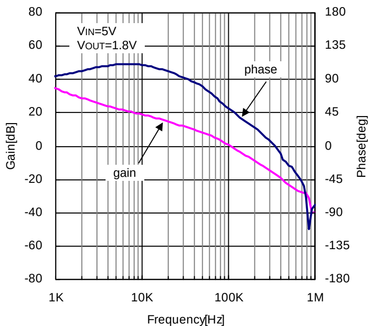
Figure 25. Closed Loop Response ( V_{IN}=5V , V_{OUT}=1.8V , I_{OUT}=6A , L=1.5\mu H , R3=6.8k\Omega , C6=5600pF , C14=100pF )
