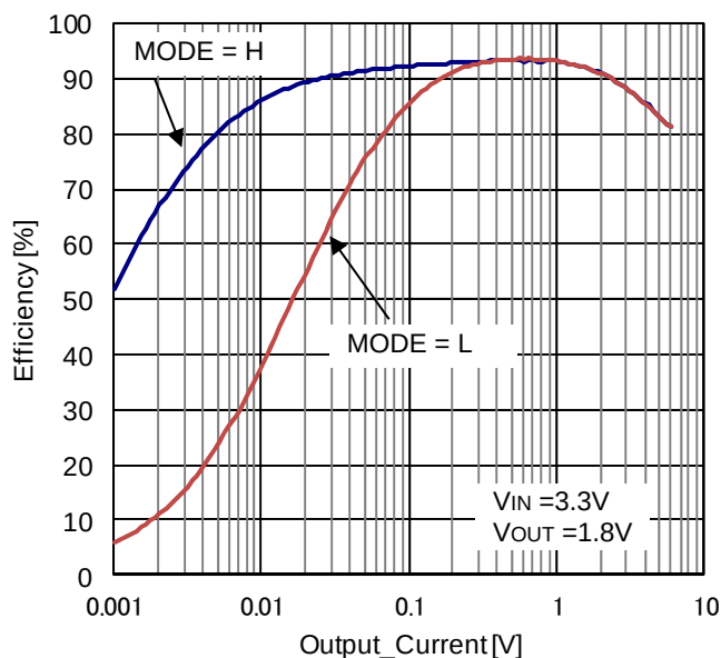
Figure 23. Efficiency vs Load Current ( V_{IN}=3.3V , V_{OUT}=1.8V , L=1.0\mu H )
