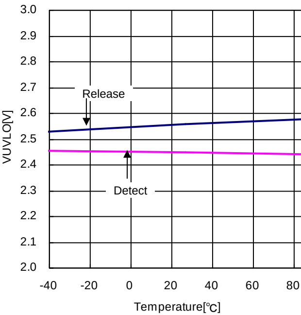
Figure 19. UVLO Threshold vs Temperature
