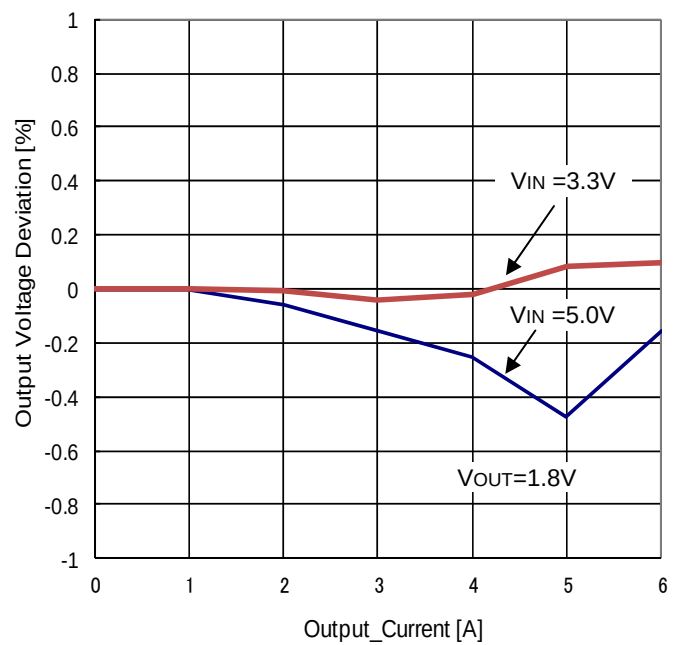
Figure 38. Load Regulation vs Load Current
