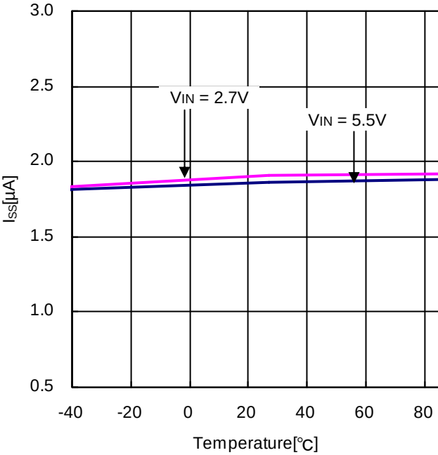
Figure 13. Soft Start Terminal Current vs Temperature
