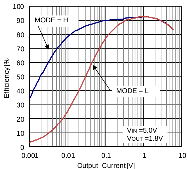
Figure 22. Efficiency vs Load Current ( V_{IN}=5V , V_{OUT}=1.8V , L=1.5\mu H )
