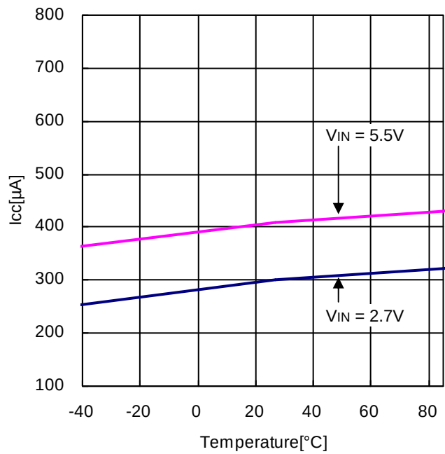
Figure 4. Operating Current vs Temperature
