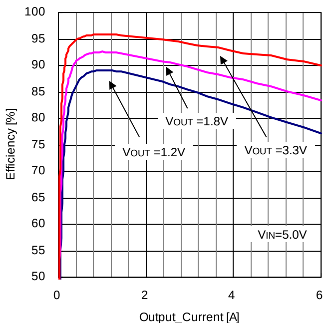
Figure 24. Efficiency vs Load Current ( V_{IN}=5.0V , MODE=5.0V )
