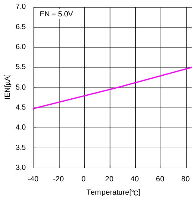
Figure 21. EN Input Current vs Temperature
