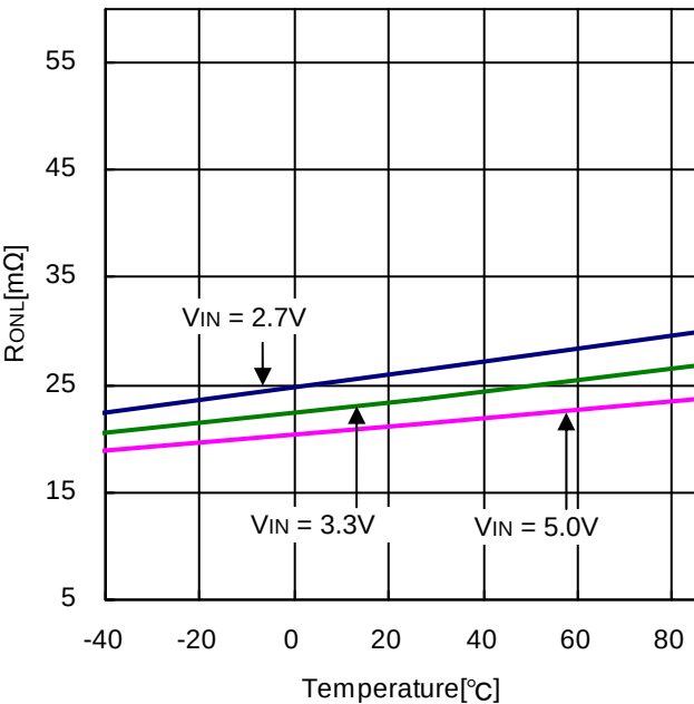
Figure 15. Low-side FET ON-Resistance vs Temperature
