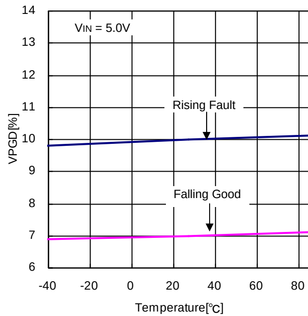
Figure 17. PGD Rising Voltage vs Temperature
