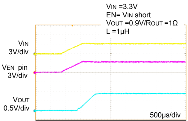
Figure 10. Start up (with VIN UVLO)
