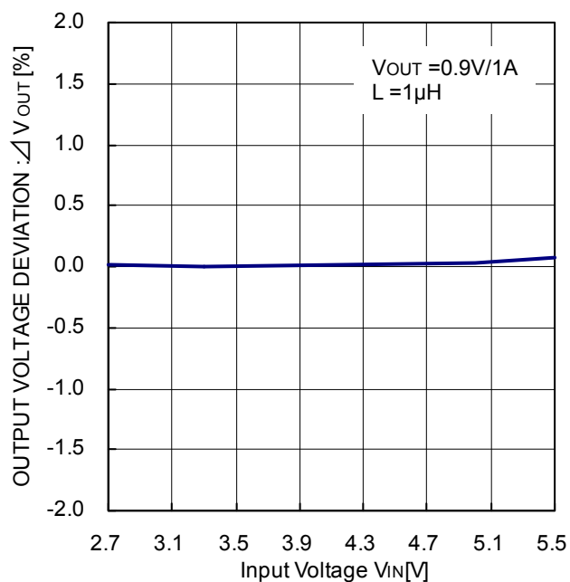
Figure 26. Output variation (Line regulation)
