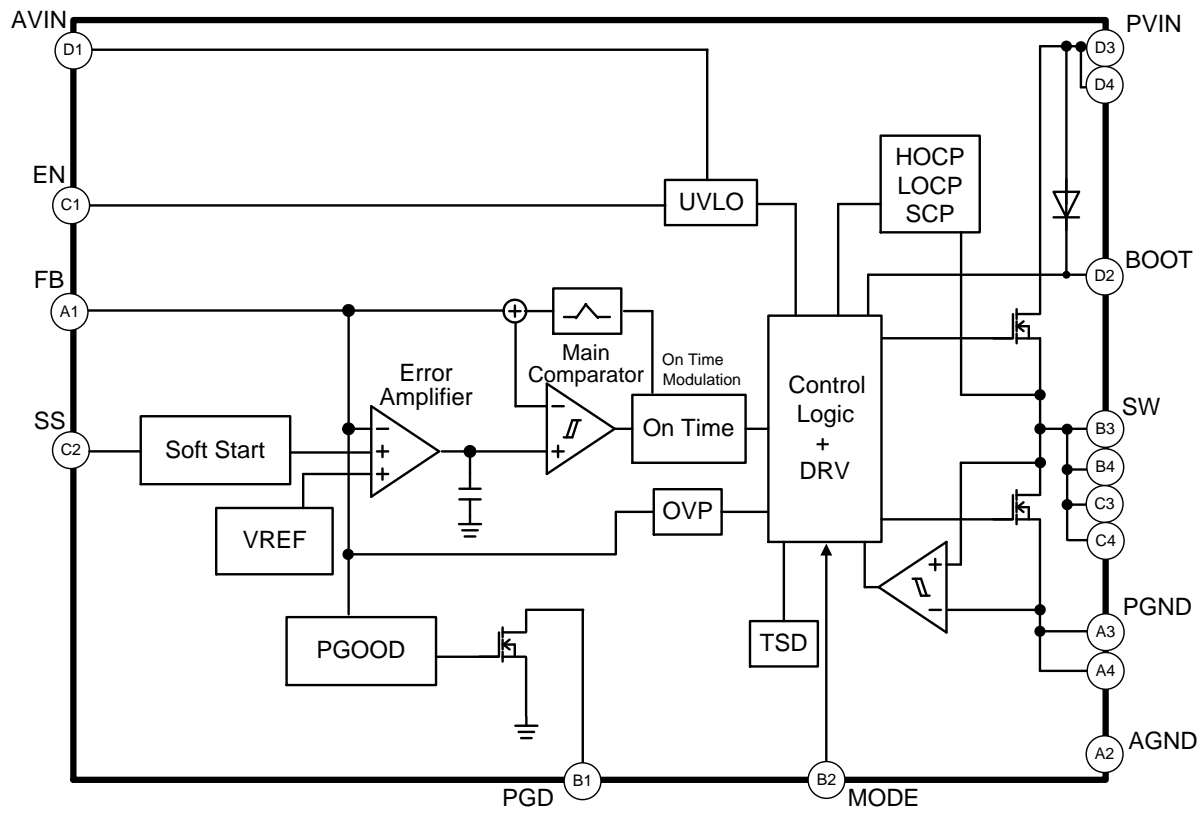
Figure 3. Block Diagram
