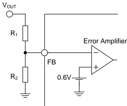
Figure 74. Feedback Resistor Circuit
