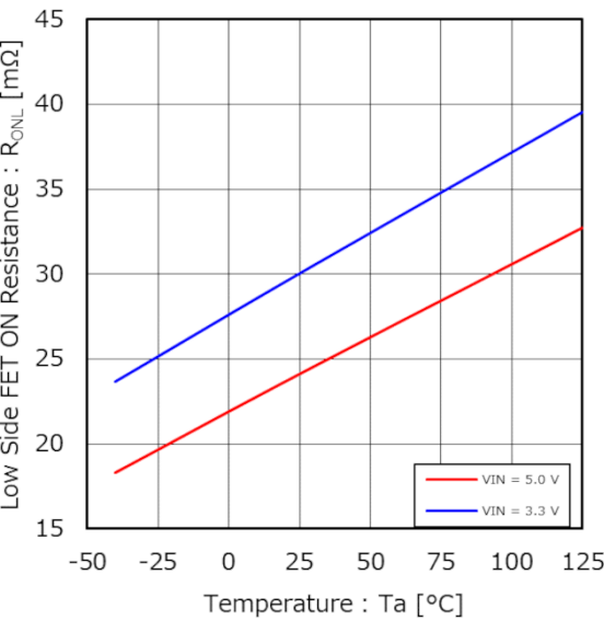
Figure 11. Low Side FET ON Resistance vs Temperature
