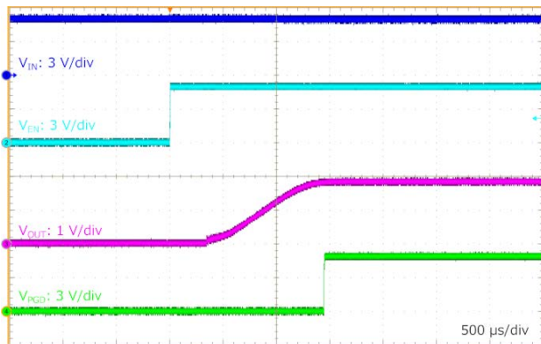
Figure 58. EN Start-up at R_{Load} = 0.45\ \Omega ( V_{IN} = 5.0\text{ V} , V_{OUT} = 1.8\text{ V} , V_{EN} = 0\text{ V to } 5\text{ V} )
