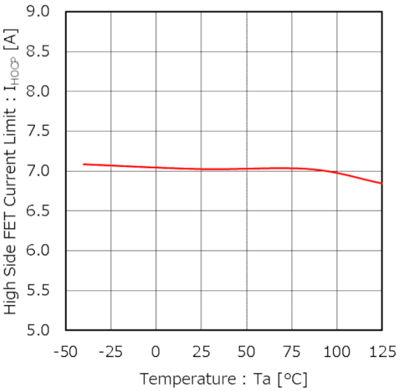
Figure 12. High Side FET Current Limit vs Temperature
