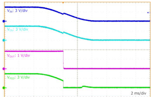
Figure 63. VIN Shutdown at R_{Load} = 0.45\ \Omega ( V_{IN} = V_{EN} = 5\text{ V} to 0\text{ V} , V_{OUT} = 1.8\text{ V} )
