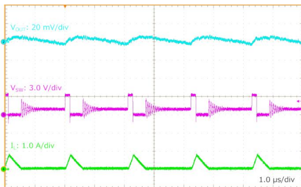
Figure 46. Output Ripple Voltage ( V_{IN} = 3.3\text{ V} , V_{OUT} = 0.9\text{ V} , I_{OUT} = 0.1\text{ A} )
