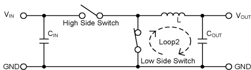
Figure 70-b. Current Path when High Side Switch = OFF, Low Side Switch = ON
