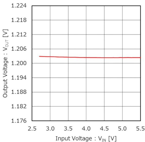
Figure 42. Output Voltage vs Input Voltage (Line Regulation) ( V_{OUT} = 1.2\text{ V} , I_{OUT} = 1.0\text{ A} )
