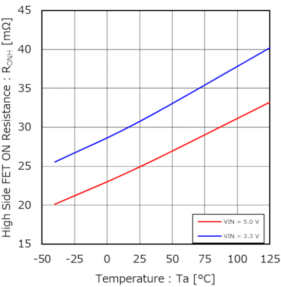
Figure 10. High Side FET ON Resistance vs Temperature
