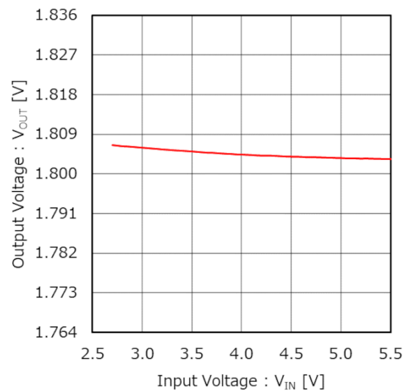
Figure 43. Output Voltage vs Input Voltage (Line Regulation) ( V_{OUT} = 1.8\text{ V} , I_{OUT} = 1.0\text{ A} )
