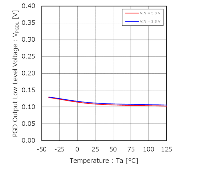
Figure 16. PGD Output Low Level Voltage vs Temperature
