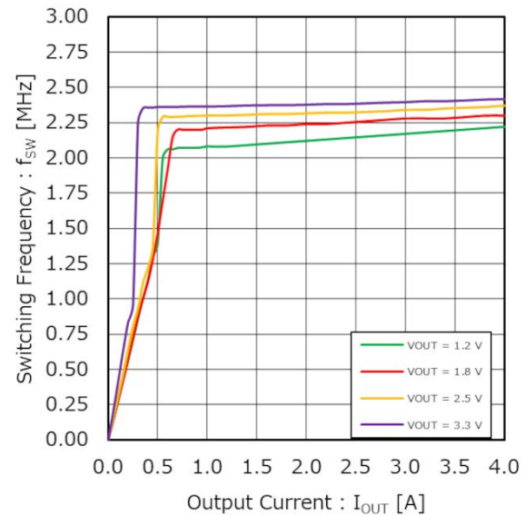
Figure 41. Switching Frequency vs Output Current ( V_{IN} = 5.0\text{ V} )
