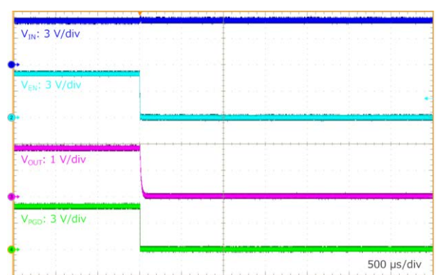
Figure 59. EN Shutdown at R_{Load} = 0.45\ \Omega ( V_{IN} = 5.0\text{ V} , V_{OUT} = 1.8\text{ V} , V_{EN} = 5\text{ V to } 0\text{ V} )
