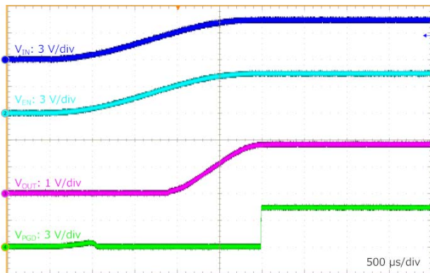
Figure 62. VIN Start-up at R_{Load} = 0.45\ \Omega ( V_{IN} = V_{EN} = 0\text{ V} to 5\text{ V} , V_{OUT} = 1.8\text{ V} )
