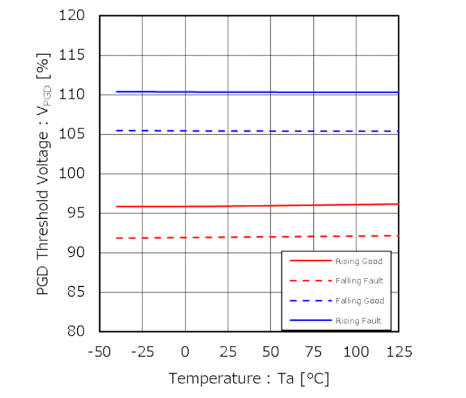
Figure 15. PGD Threshold Voltage vs Temperature
