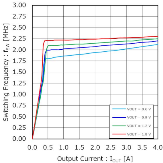
Figure 40. Switching Frequency vs Output Current ( V_{IN} = 3.3\text{ V} )
