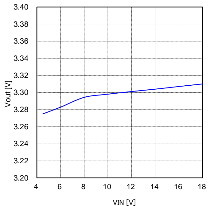
Figure 9. Line Regulation (Vout=3.3V, L=3.3μH, Cout=44μF, Iout=0A)
